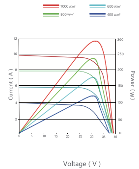
Flash Test Mode Tested by Source Simulator (285W)
