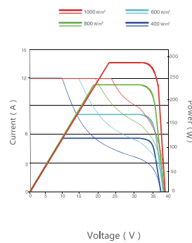
MPPT Mode Simulated Real Behavior (285W)
