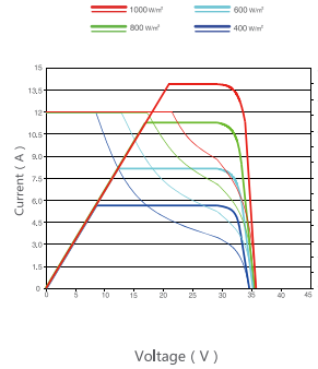
MPPT Mode Simulated Real Behavior (260W)
