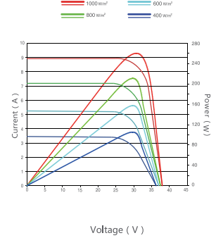
Flash Test Mode Tested by Source Simulator (260W)
